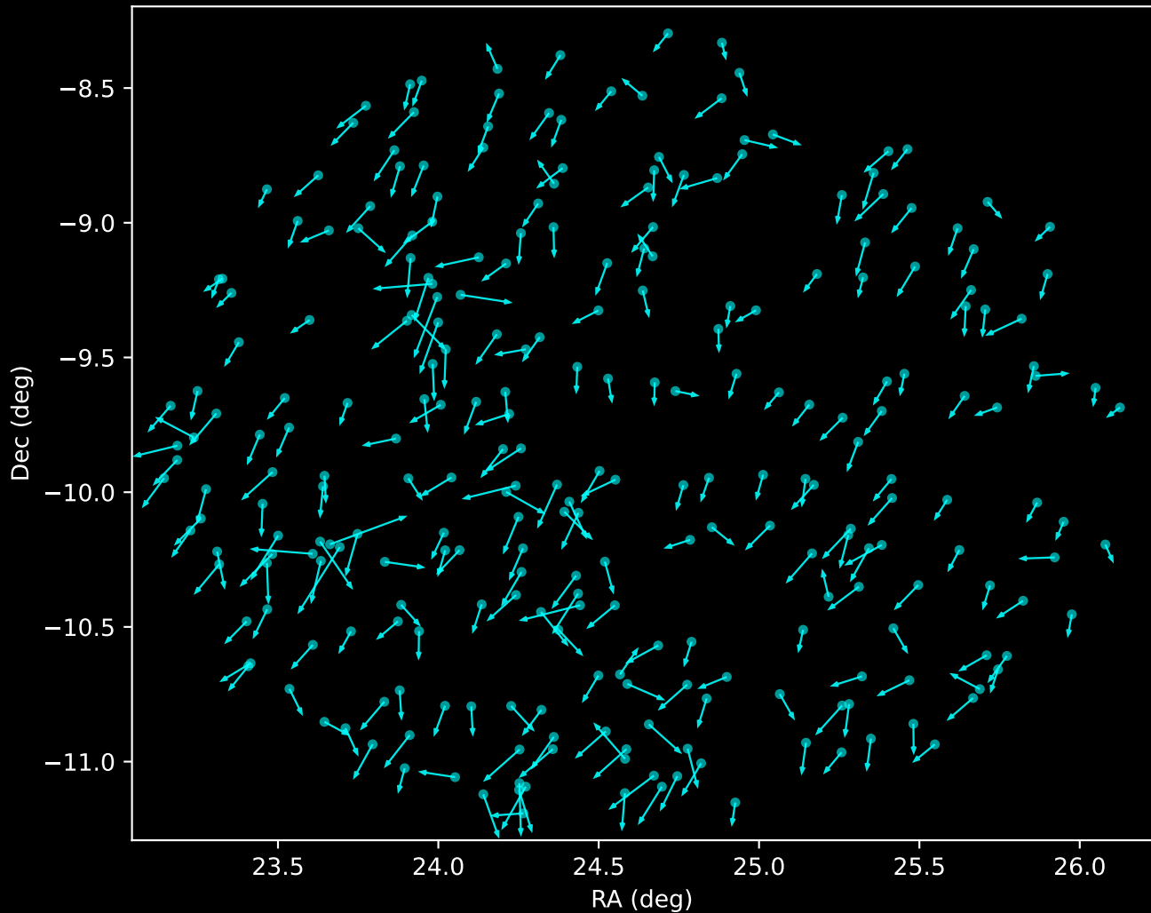
APOGEE DR17 Noise Stream Proper Motion Vectors (n=265)
