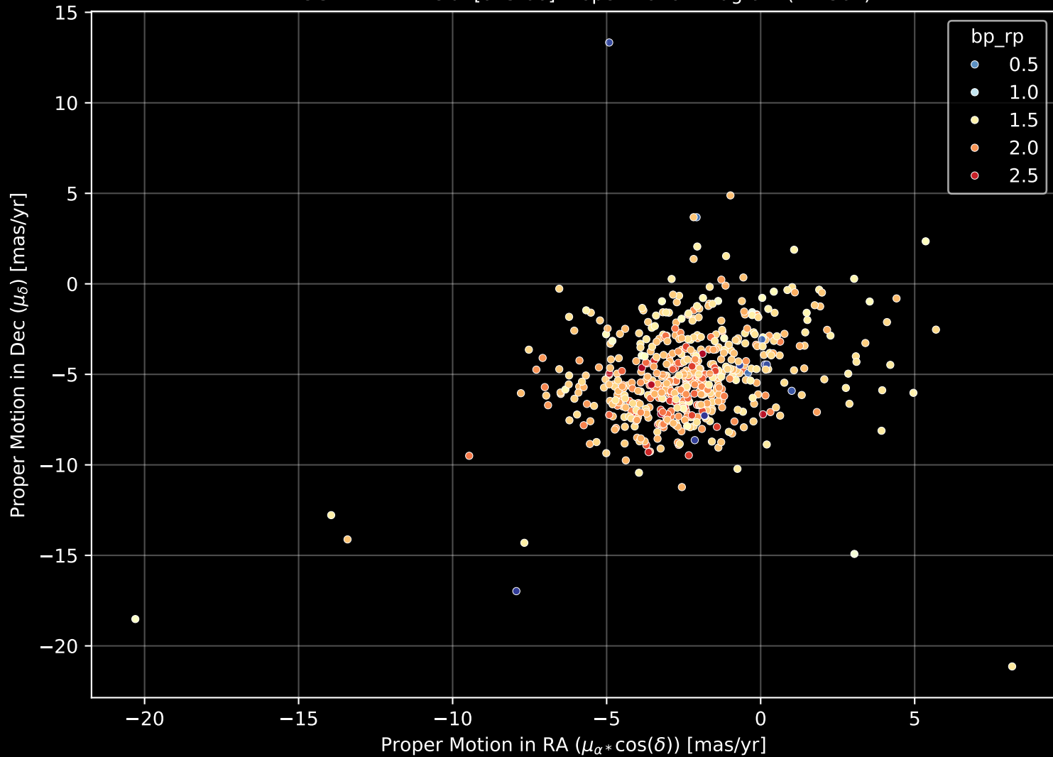
APOGEE DR17 Field: [025-06] Proper Motion Diagram (n= 561)
