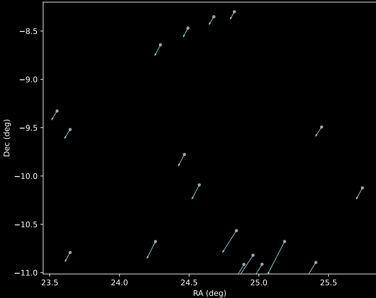
APOGEE DR17 Cluster 19 Proper Motion Vectors (n=18)
