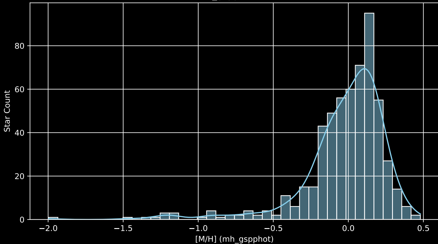
APOGEE DR17 Field: [025-06 [M/H] (mh_gspphot) (n= 557)
