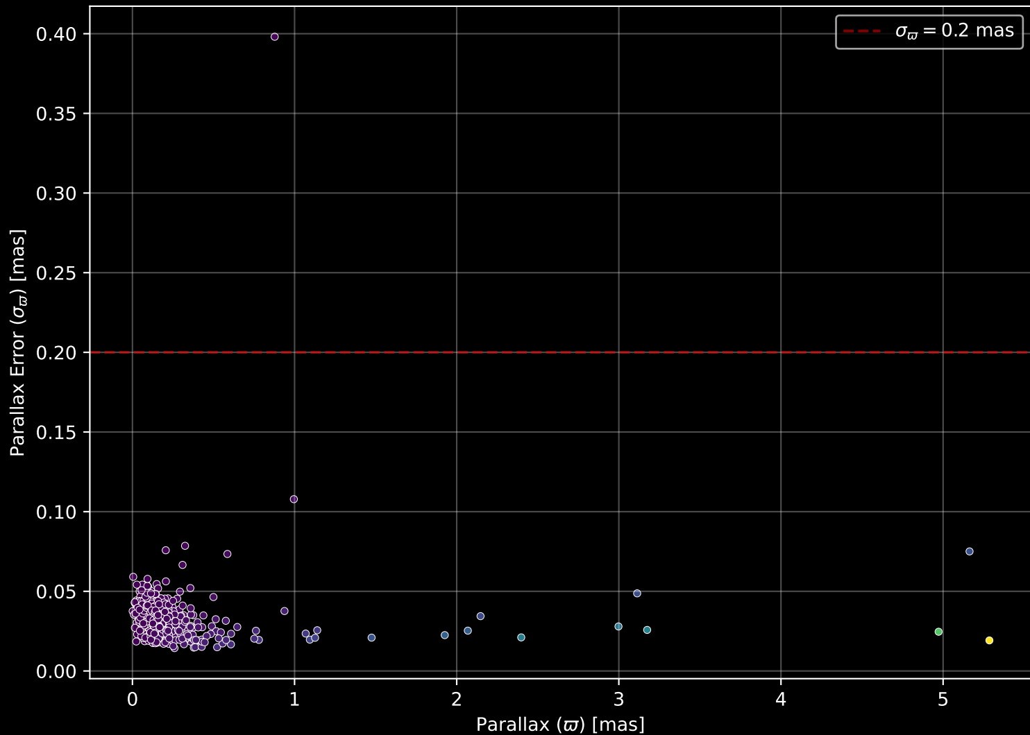
APOGEE DR17 Field: [025-06] Parallax Quality (n= 561)
