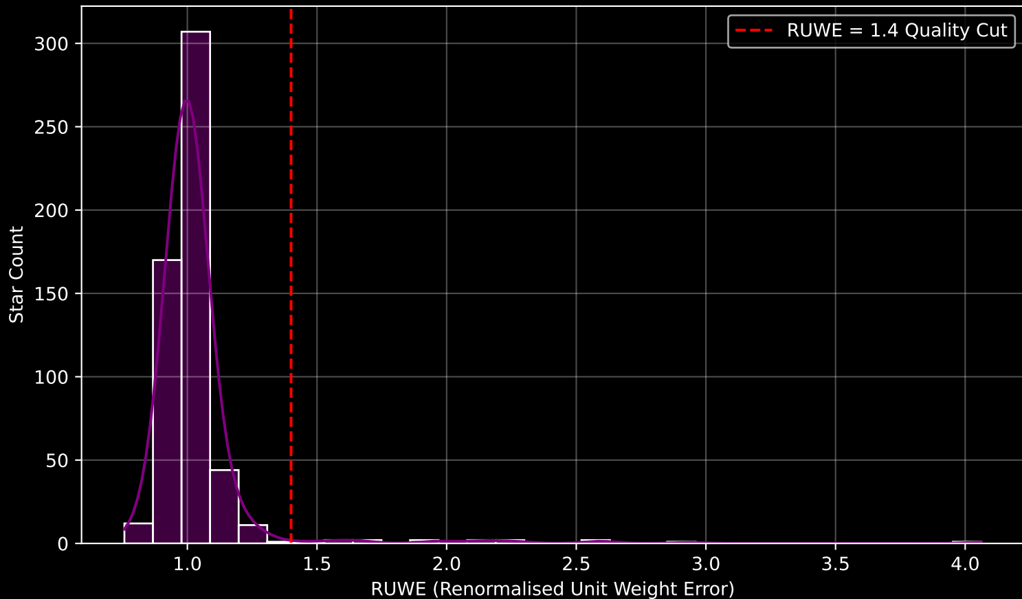
GAPOGEE DR17 Field [025-06] RUWE Distribution (n= 560)
